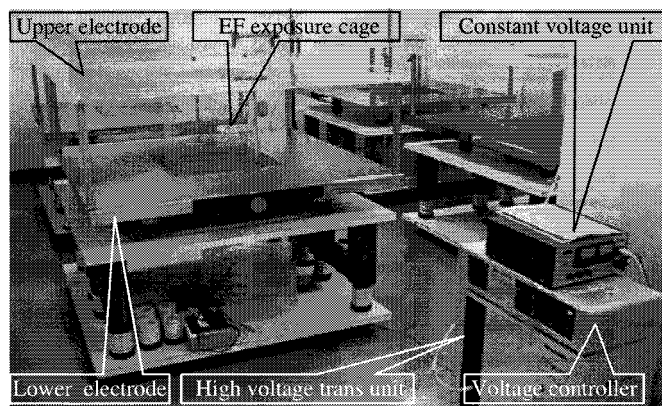
Fig. 1. The Electric Field (EF) Exposure System. A cylindrical plastic cage is placed between one upper and three lower stainless steel electrodes. The cylindrical cage has slits (length: 100 mm; width: 5 mm) at 5 mm intervals. The slits prevent contamination due to feces and saliva from disturbing the formation of a stable EF.
